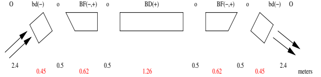
Figure 1: Isochronous cell.
