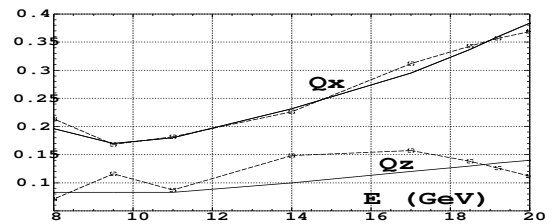
Figure 4: Cell tunes vs. energy obtained either from matrix method or (markers) from ray-tracing.
