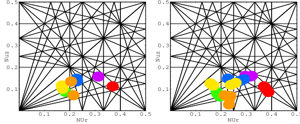
Figure 7: Amplitude detuning and its energy dependence.
