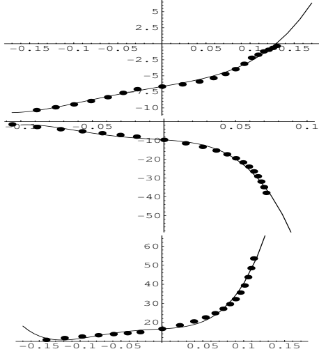
Figure 5: Field strengths ( m^{-2} ) as a function of transverse coordinate in, respectively, bd (top), BD (middle) and BF (bottom). The dots are the design data, the solid lines represent the ray-tracing 4th degree interpolation polynomials.
