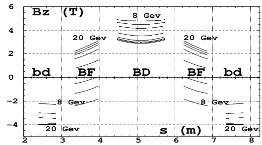
Figure 2: Magnetic field on closed orbits at various energies.
