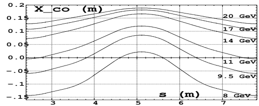
Figure 3: Closed orbits at various energies.
