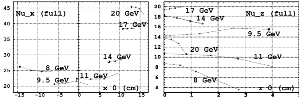
Figure 7: Amplitude detuning and its energy dependence.
