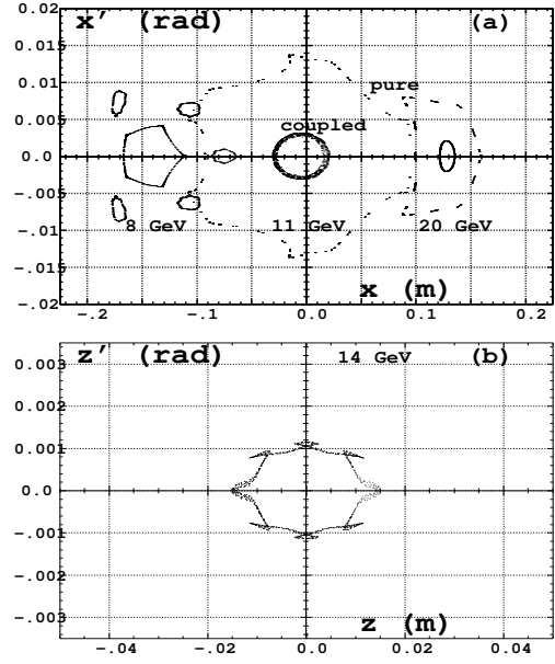
Figure 6: Stability limits. (a) in horizontal phase-space, at 8, 11 and 20 GeV, either pure (the largest amplitude) or with paraxial z component (“coupled”, the smallest amplitude). (b) vertical phase-space, at 14 GeV, with initial (x, x') taken on closed orbit.
