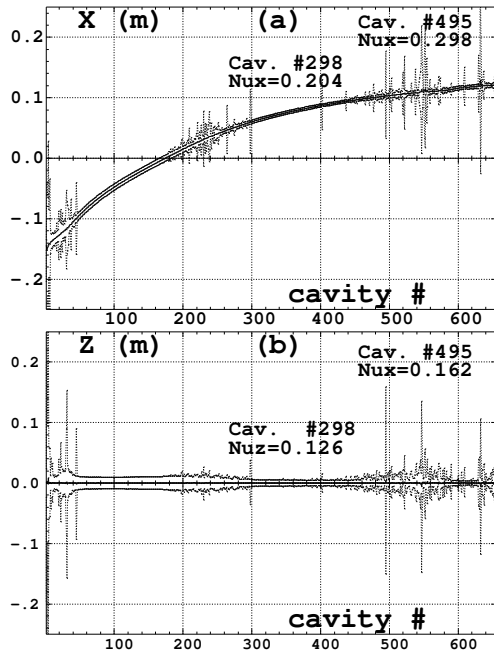
Figure 9: Beam centroid position and envelopes.
