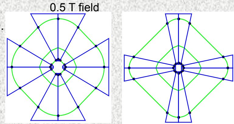
Low-energy cyclotron (left) and equivalent FFAG (right)
