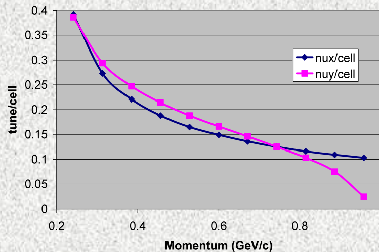
tune variations in a nonscaling FFAG
