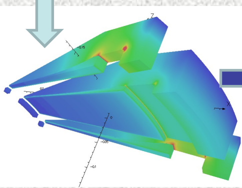
TOSCA Magnet Design and Field profiles.
