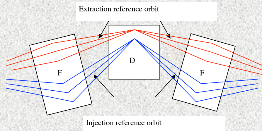
1½ cell of a nonscaling, linear-field FFAG for muon acceleration showing the compression of orbits in particular in the center magnet.
