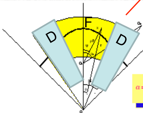
Radial Sector: example: This is a triplet DFD cell; there are also FDF, FODO and doublets. In a radial sector the D is the negative of the F field profile, but shorter.
