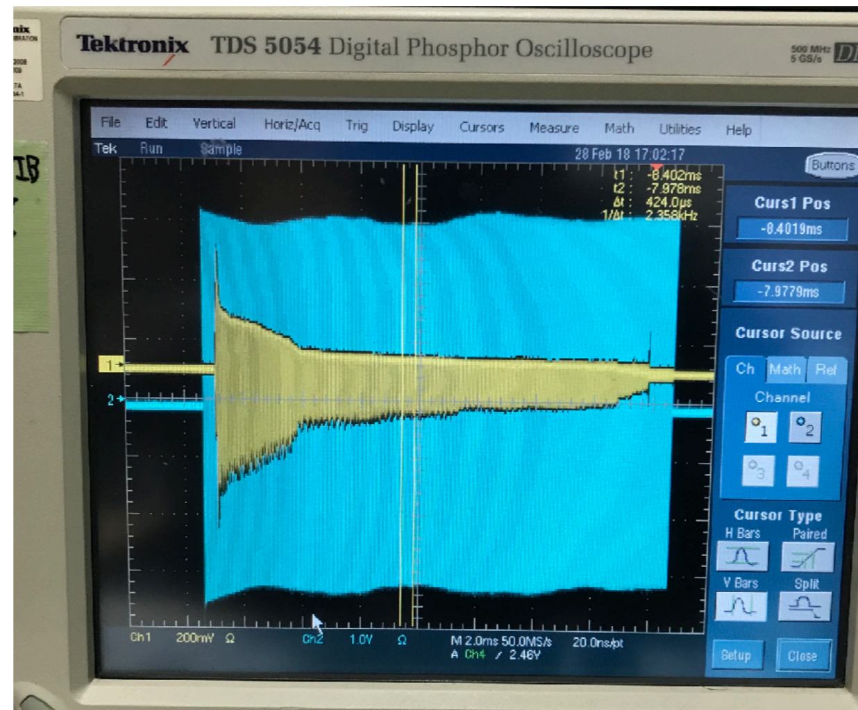
Fig.1 main ring bunch monitor signal 2018.2.28
