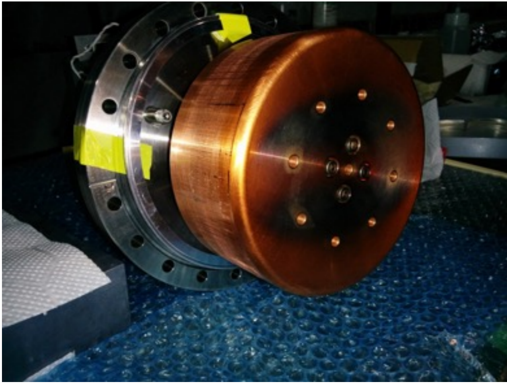
slug tuner pulled out of DTL1
