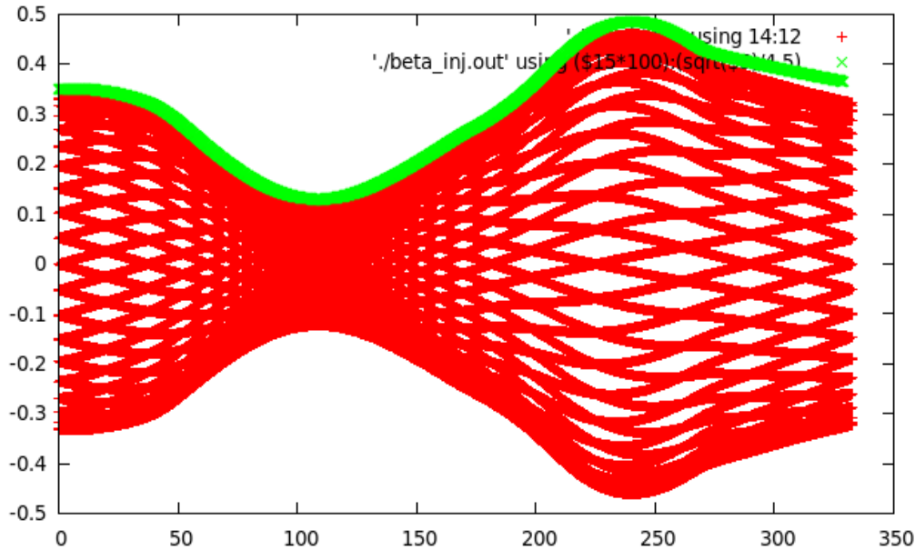
Vertical beam envelope
