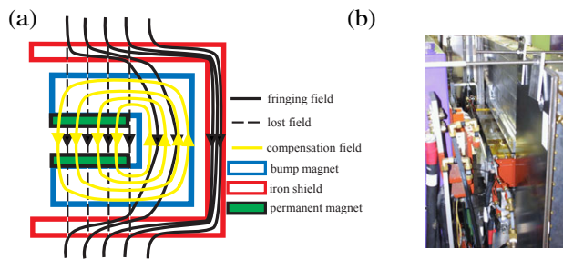
Figure 4: COD suppression magnets (a) Schematic view of Bump (b) Figure of RF COD magnet COD suppression magnet
